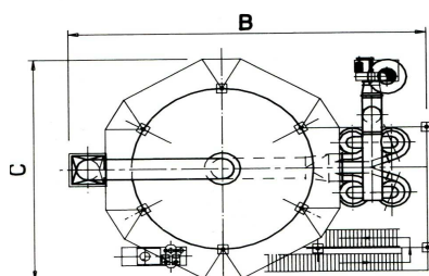
Spray dryer with pressure nozzles type with axial distribution of the hot air.
